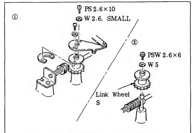
Fig. 6-66. Replacement of Link Wheel S
